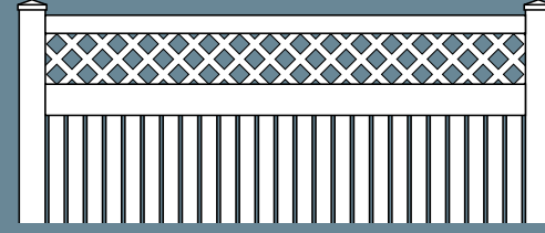
Garrett Traditional Diagonal Lattice - 2 3/4" Openings 3" Semi Privacy Picket
