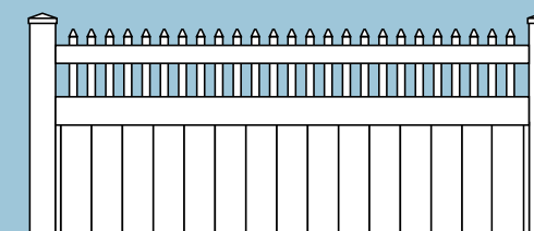
Worcester 7/8" x 1 1/2" Open Straight Top with Approximately 2" Air Space Picket Through Top Rail
